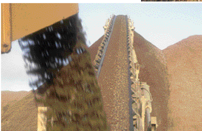
The discharge conveyor from a crushing plant is in the foreground. Notice how badly segregated the material is as it is carried up the stockpile on a belt stacker. This invariably leads to problems illustrated in the following two photos.
